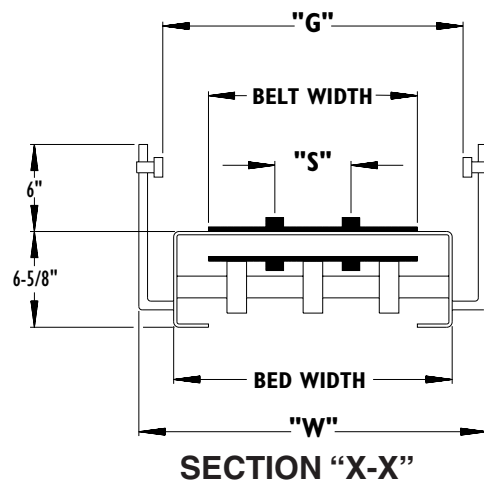
SHOWN WITH OPTIONAL ADJUSTABLE CHANNEL GUARD RAILS
