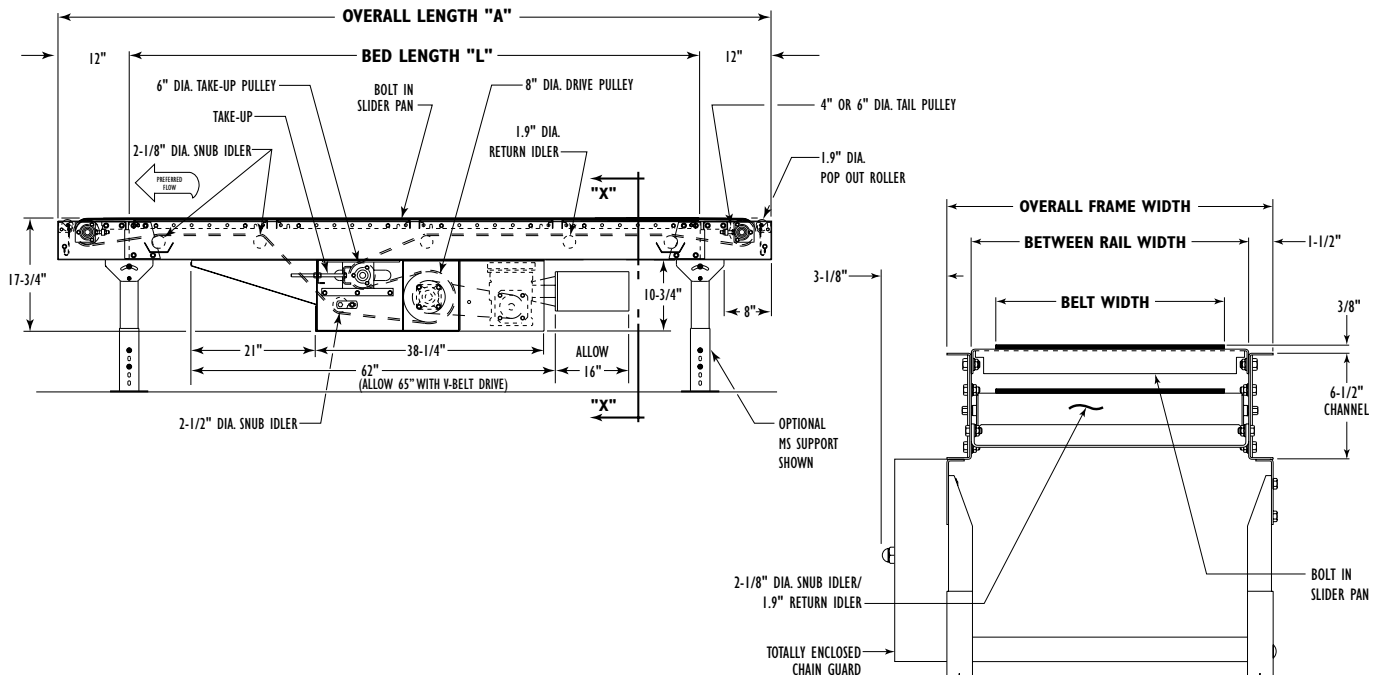
SECTION "X-X"
