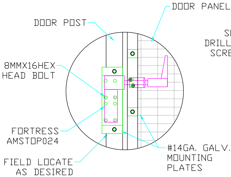
FRONT DETAIL FORTRESS AMSTOP024
