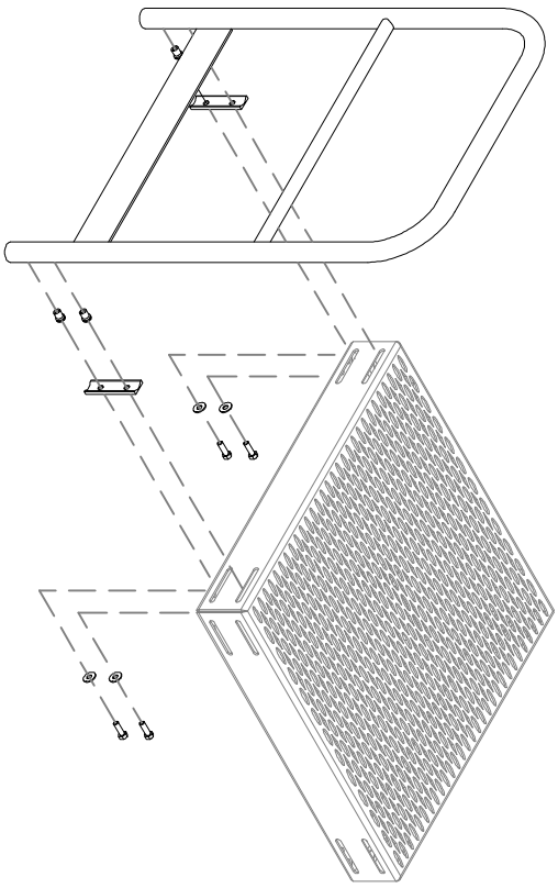
TYPICAL BOLTED CONNECTION
