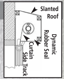
Face Mount
