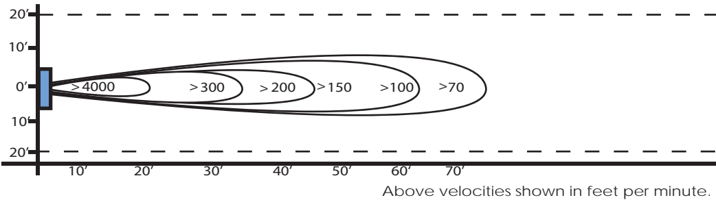
HVTC High Velocity Fan Air Flow Pattern
