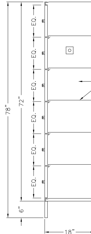
SECTION @ WALL
