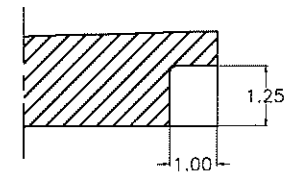
SECTION A-A (FEMALE END) SCALE 1=2
