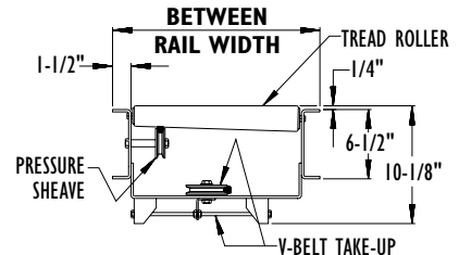
VIEW "Y-Y"
