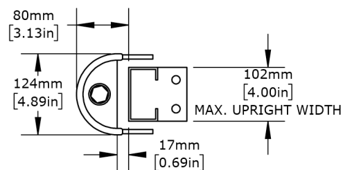
Top View - Standard Racks SCALE: 1:8
