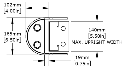
Top View - Wide Racks SCALE: 1:8
