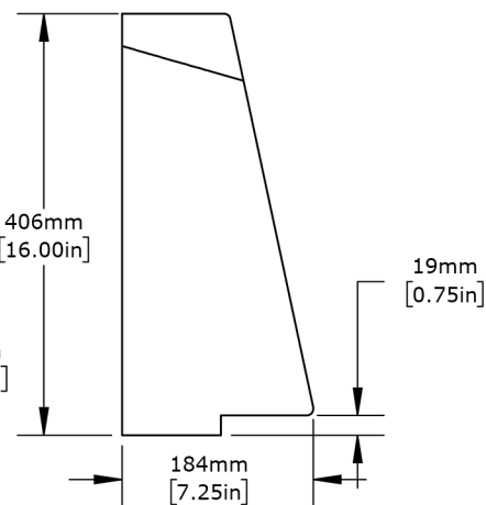
16" Shock Absorbing Rack Guard for Wide Racks SCALE: 1:8
