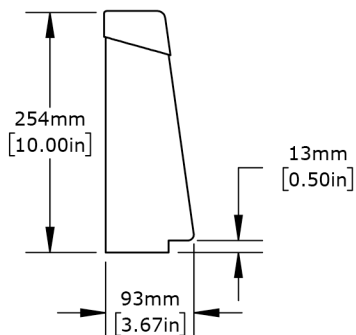
10" Shock Absorbing Rack Guard for Standard Racks SCALE: 1:8
