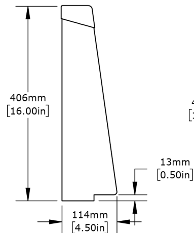
16" Shock Absorbing Rack Guard for Standard Racks SCALE: 1:8
