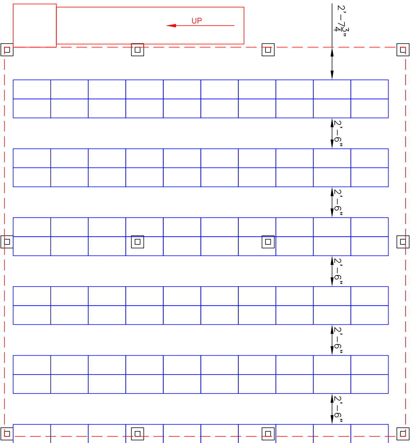
FLOOR LEVEL – OPTION 2 110 SHELVING UNITS
