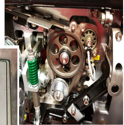
Strapping Head
