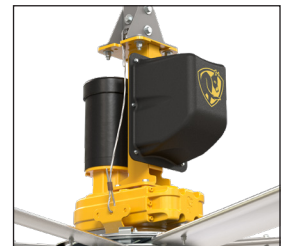
Onboard VFD and NitroSeal Drive Gearbox
