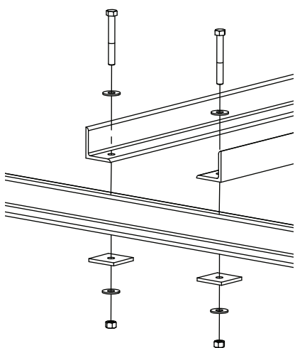
Angle Iron Hardware (single angle irons)
