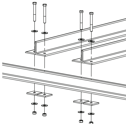
Angle Iron Hardware (double angle irons)
