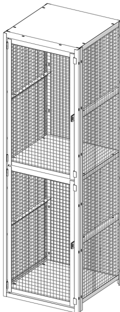
DOUBLE TIER
