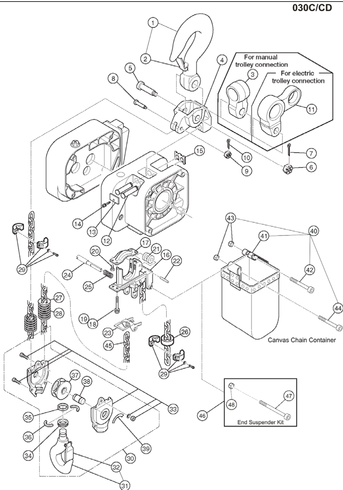
Figure 9-3-5 Hook and Chain Parts
