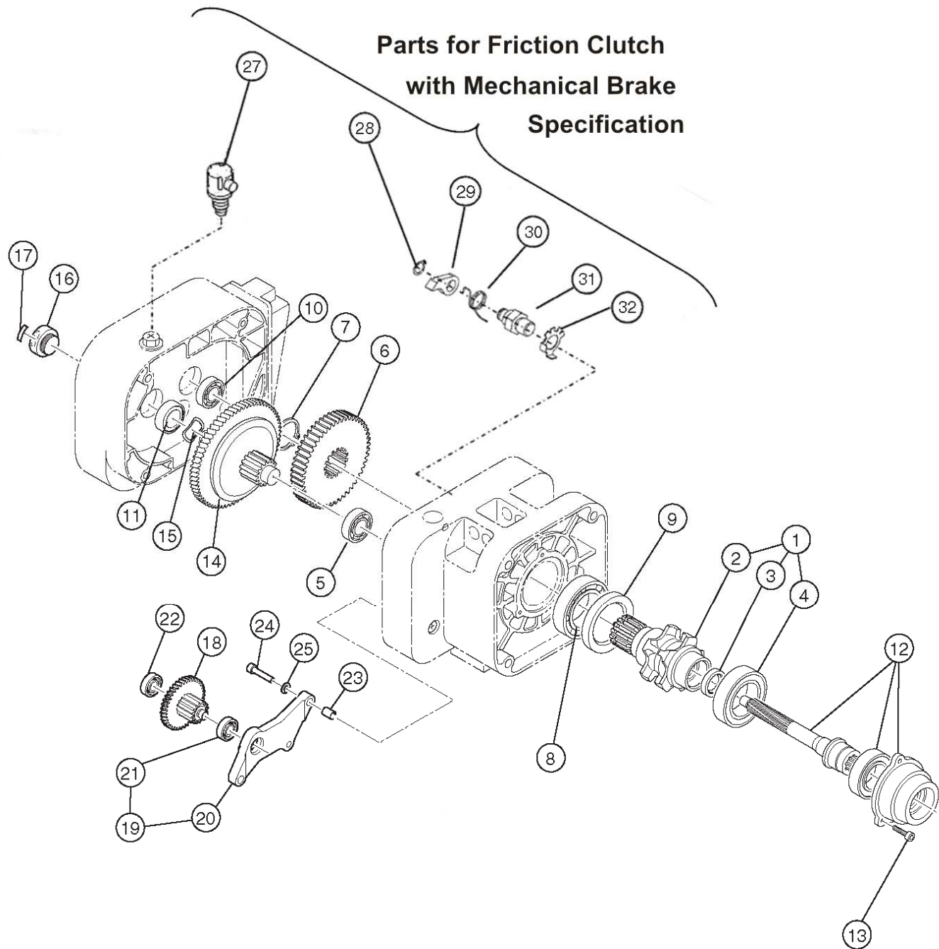
Figure 9-2-1 Gearing Parts
