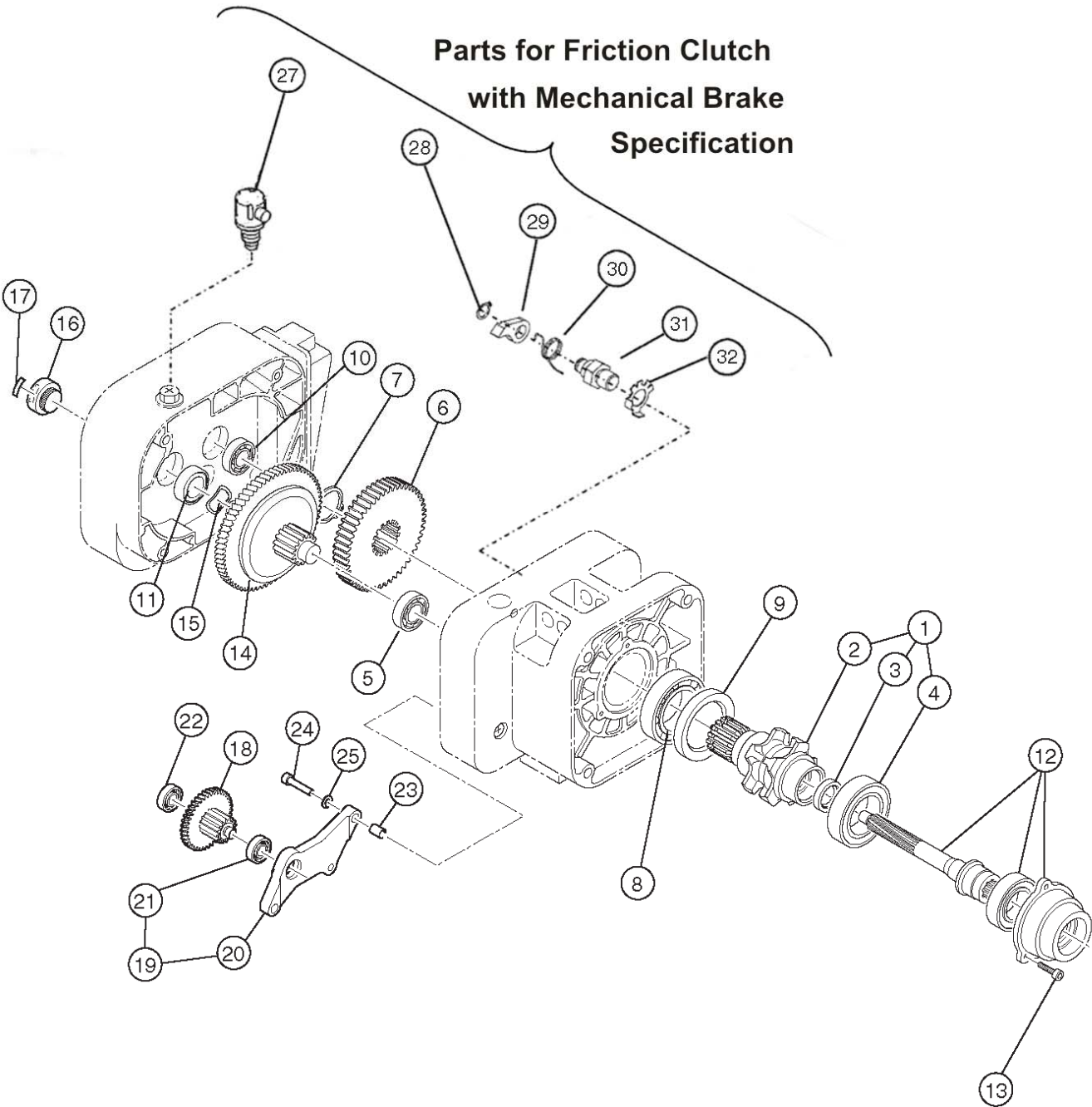
Figure 9-2-2 Gearing Parts
