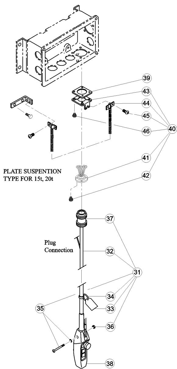
Figure 9-7-1 Power Supply and Pendant Parts (Plug Connection)
