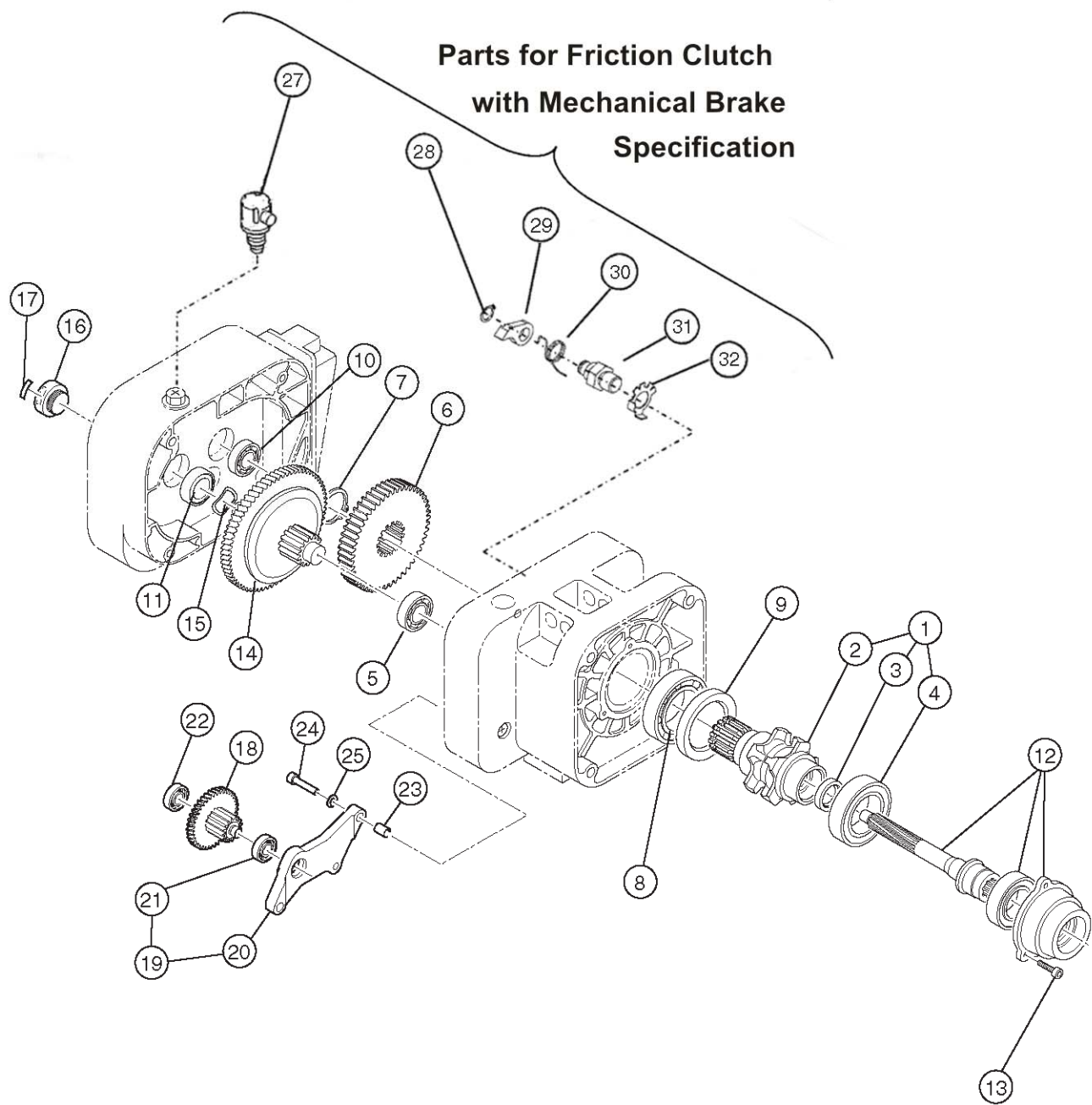
Figure 9-2-1 Gearing Parts
