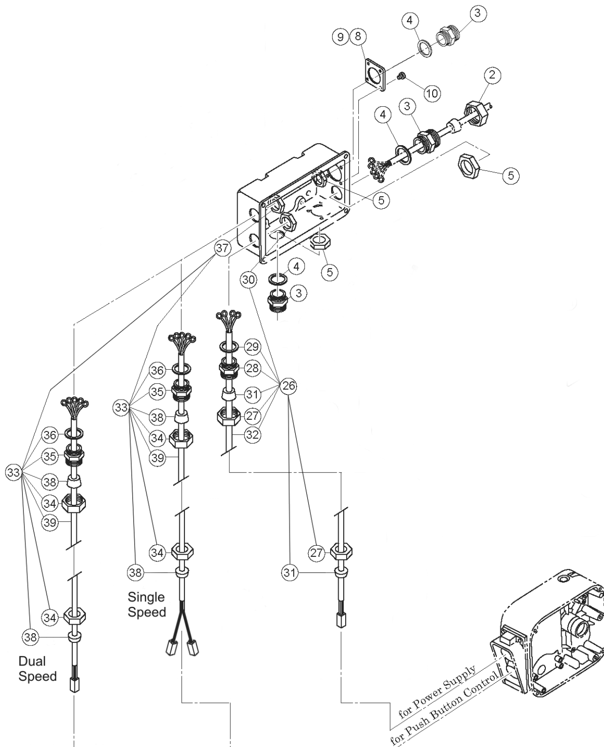
Figure 9-1-3 Electric Parts (Direct Connection)
