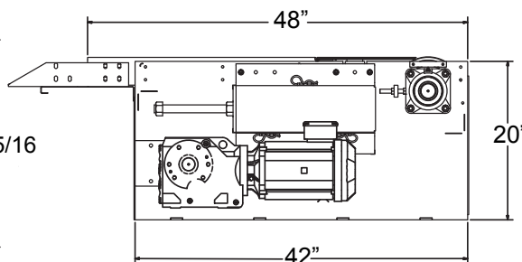
DRI-34 (8 5/8" Diameter Drive Pulley)
