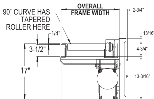
SECTION X-X
