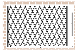
FIXED BOTTOM TRACK - Single Gate Max Width 6' | Max Height 8'6"
