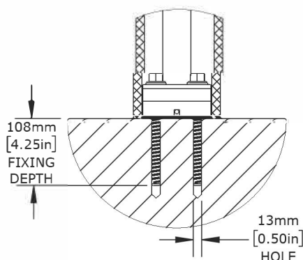
FlexCore 4 Fixing Detail
