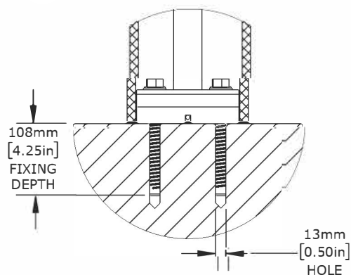
FlexCore 6 Fixing Detail
