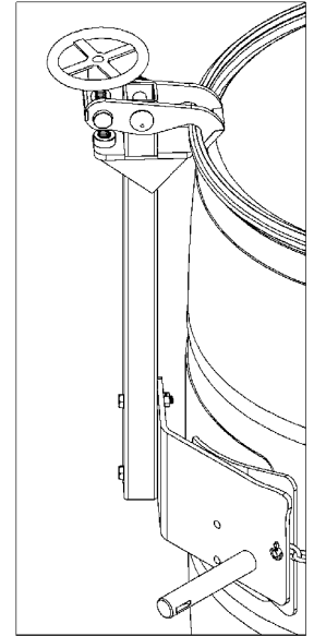
Figure 2.2 Plastic drum being lifted with Kit # 4560-P Top Rim Clamp Assembly installed.
