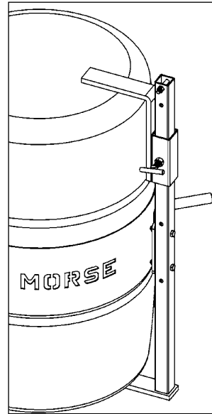
Figure 2.1 Plastic drum being lifted with Kit # 4556-P Bracket Assembly installed.
