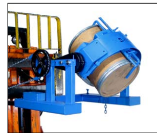
Forklift-Karrier with 55/30-16
