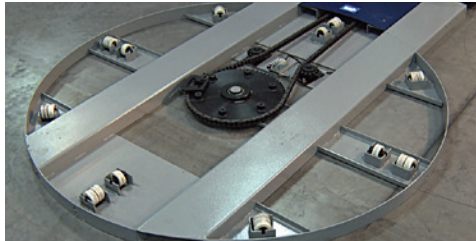
Structural steel plate and tube is used to provide a robust and durable base. Soft-start rotation prevents unstable loads from toppling when cycle begins.
