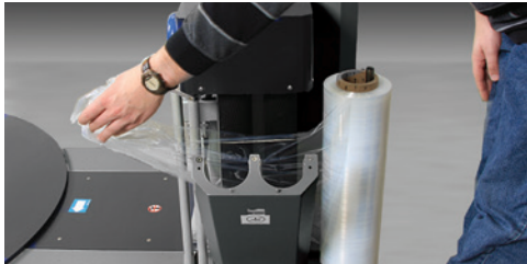
Loading film is fast and easy: open the hinged door, pull the film tail through, and close the door. Power is disconnected when the door is opened.
