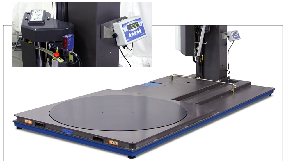
Scale readout can be permanently or magnetically mounted to the mast of the machine (top photo). The scale is often ordered to exactly match the measurements of the base of the wrapping machine (bottom photo).
