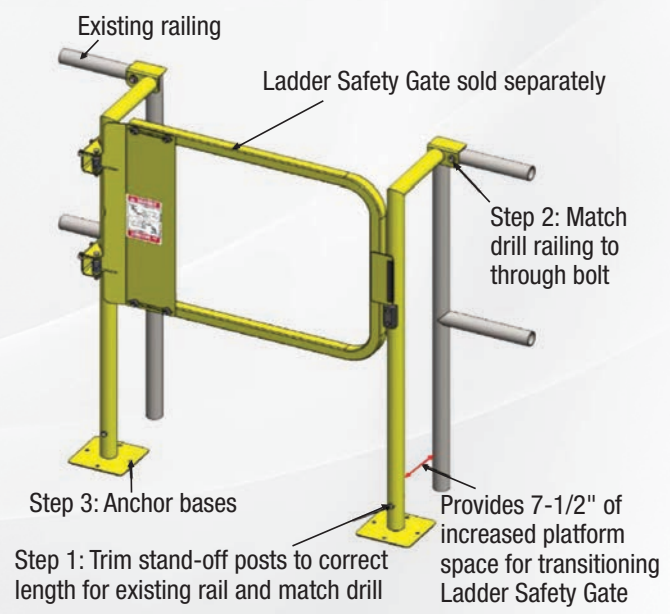
Optional Stand-Off Mounting System shown with Full Height Ladder Safety Gate
