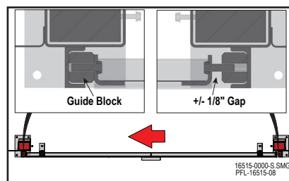
Guide Block Gap 16-91
