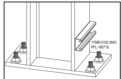
Anchor the Column Base Plates Figure 12-18
