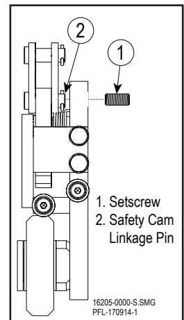
Insert Setscrew Figure 12-13
