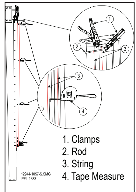
Spliced Column Alignment Figure 12-7
