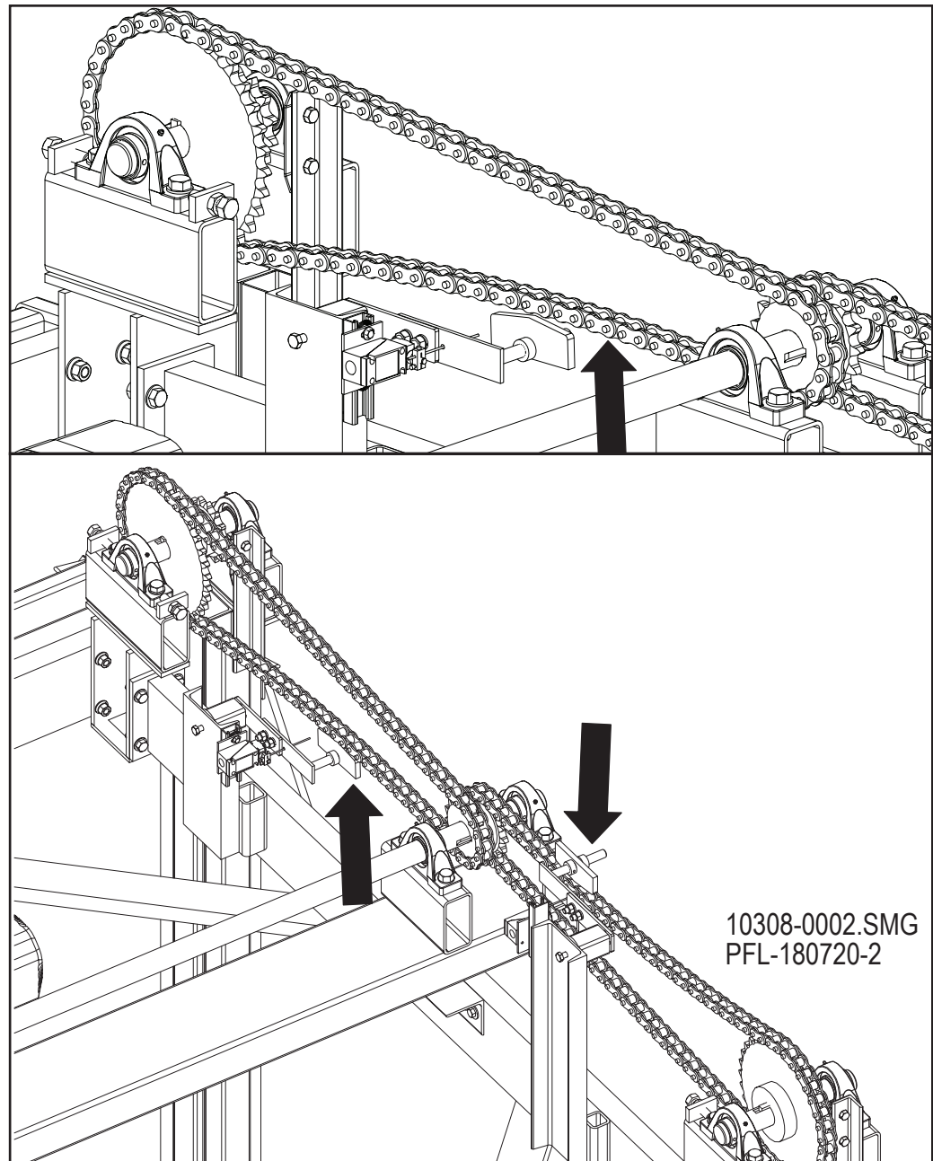
Drive Chain Tensioner Figure 12-51
