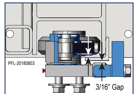
Verify Gap Figure 12-32
