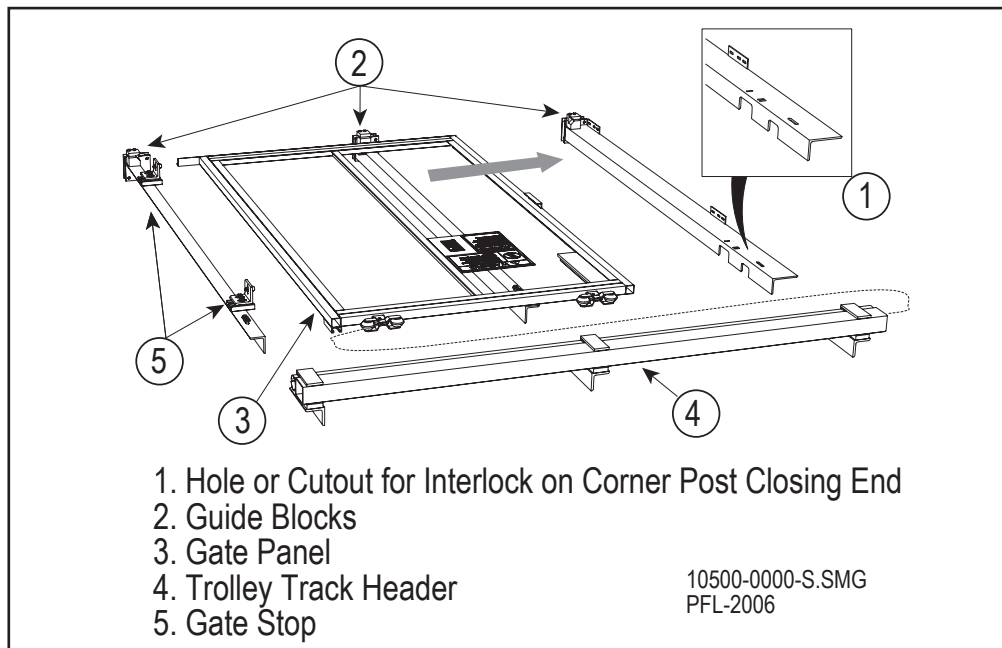
Sliding Gate Layout Figure 16-1
