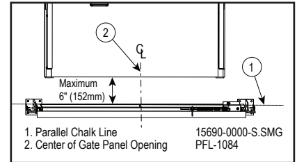
Alignment Figure 16-24
