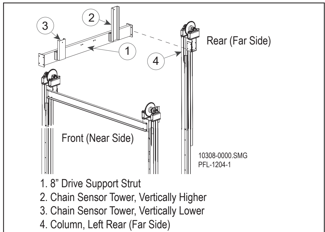
Attach Drive Support Strut Figure 12-26
