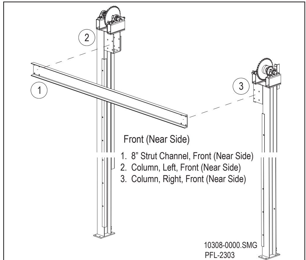
Attach Strut Channel Figure 12-21
