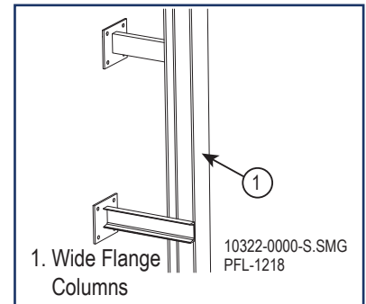
Tack Weld Bracing Figure 12-24
