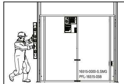
Plumb the Gate Figure 16-90
