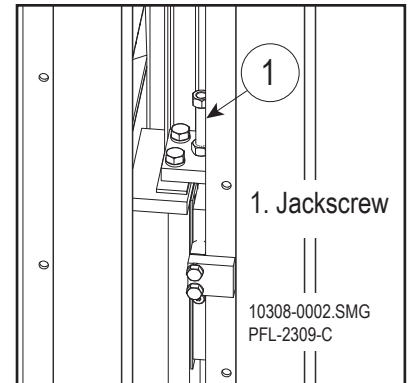
Leveling with Jackscrew Figure 12-48
