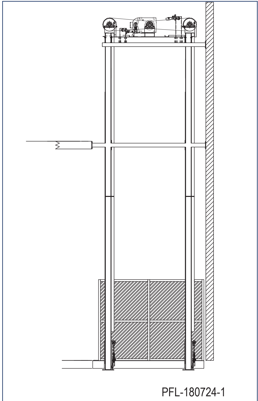
Through a Floor Figure 13-12
