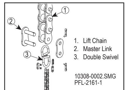
Attach the Tensioner Chain to the Lift Chain Figure 12-41
