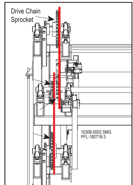
Verify Sprocket Alignment Figure 12-37
