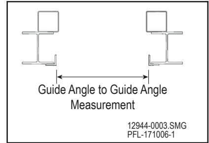
Verify Guide Angle Measurement Figure 12-22
