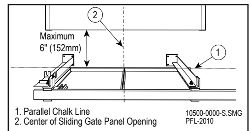
Alignment Figure 16-5
