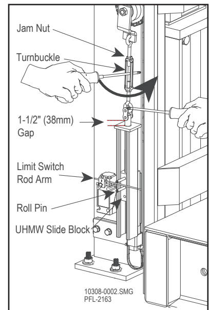
Turnbuckle Adjustment Figure 12-49
