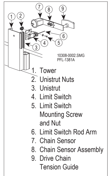
Assemble the Drive Chain Tensioner Figure 12-52
