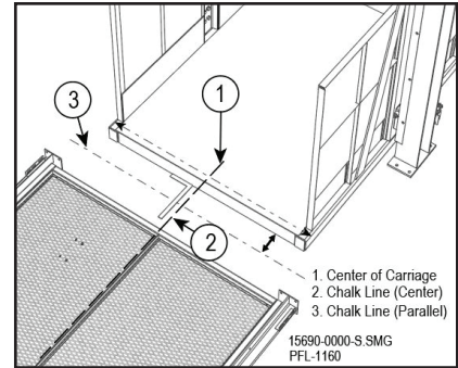
Establish Center Line Figure 16-30
