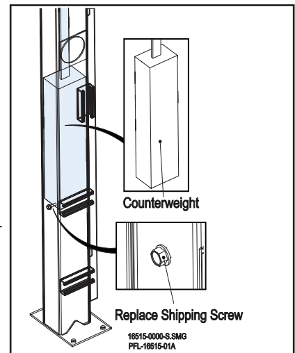
Post Assembly Counterweight Figure 16-65
