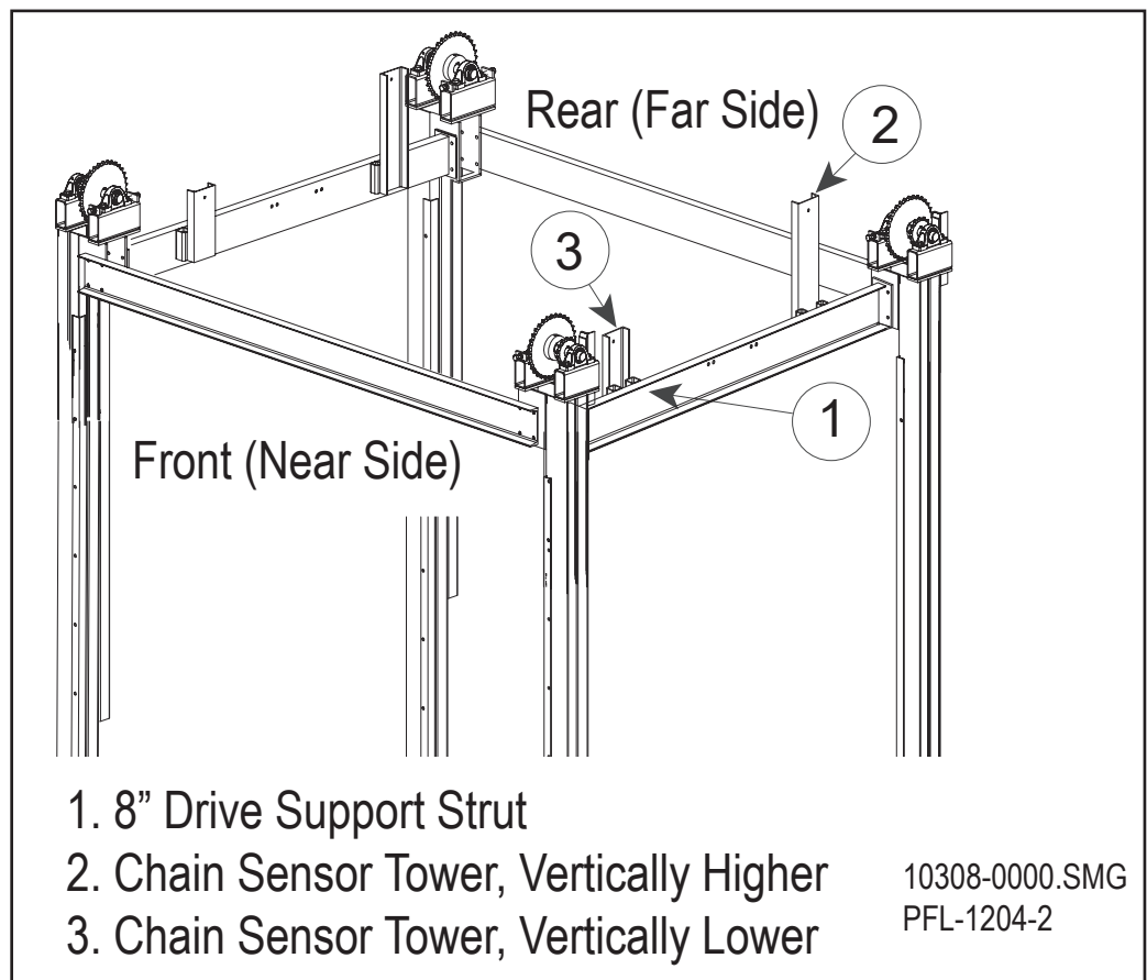
Attach Drive Support Strut Figure 12-28
