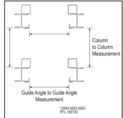
Verify Distances Figure 12-29
