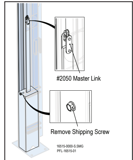
Post Assembly Counterweight Figure 16-64
