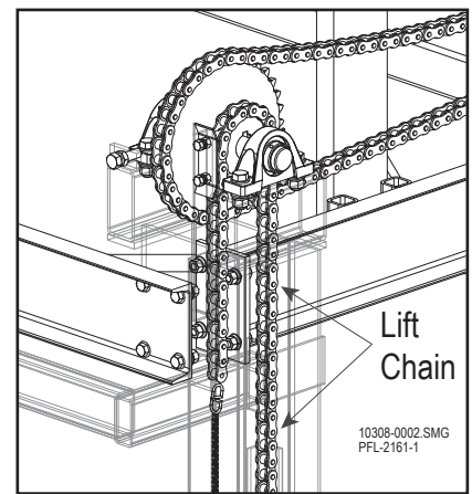
Place a Section Over the Chain Sprocket Figure 12-40
