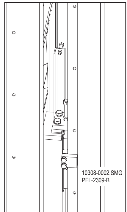
Assembled Standoff and Jackscrew Figure 12-45
