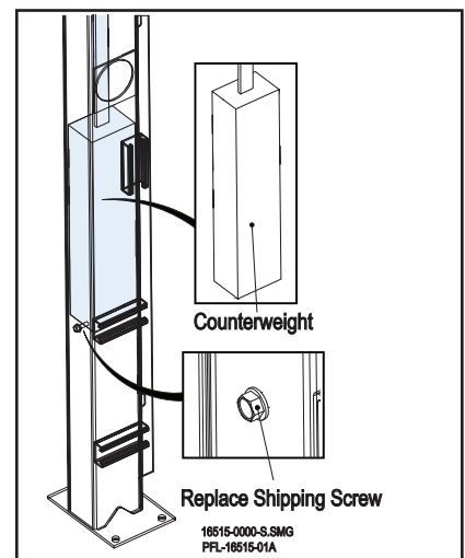
Post Assembly Counterweight Figure 16-34
