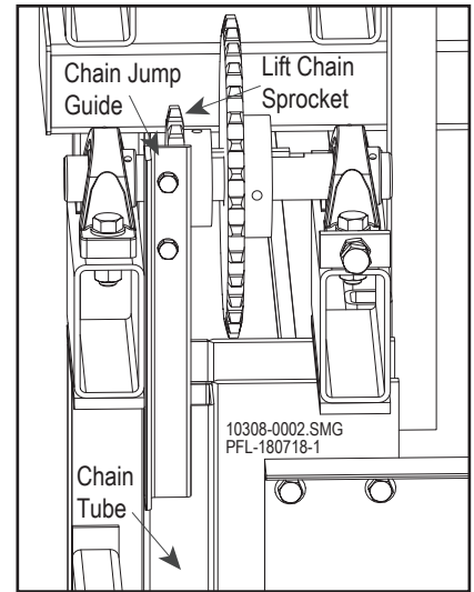
Remove Chain Jump Guide Figure 12-39
