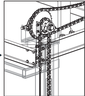
Install Lift Chains
