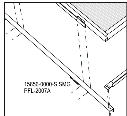
Bi-Parting Swing Gate Layout Figure 16-12
