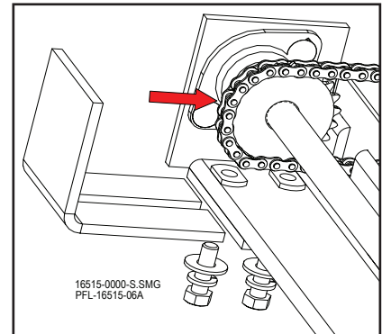
Position Center of Chain Figure 16-68
