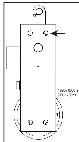
Insert Setscrew Figure 12-12
