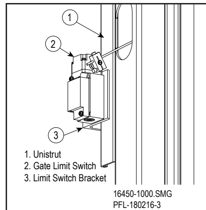
Attach Gate Limit Switch Figure 16-95
