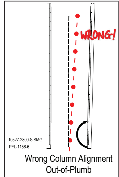
Column Alignment Out-of-Plumb Figure 12-17
