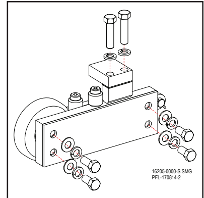
Remove Hex Head Screws Figure 12-10
