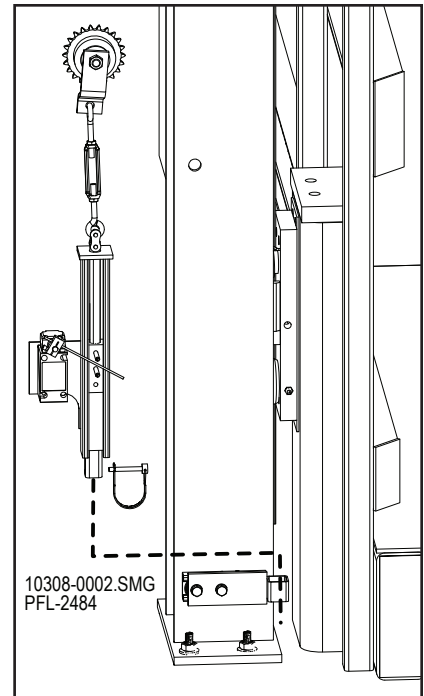
Install the Lift Chain Tensioner Assembly Figure 12-46
