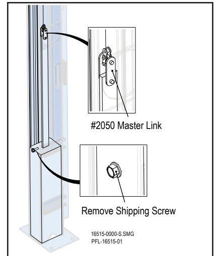
Post Assembly Counterweight Figure 16-33
