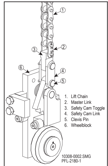
Attach the Lift Chain to the Wheelblock Figure 12-43
