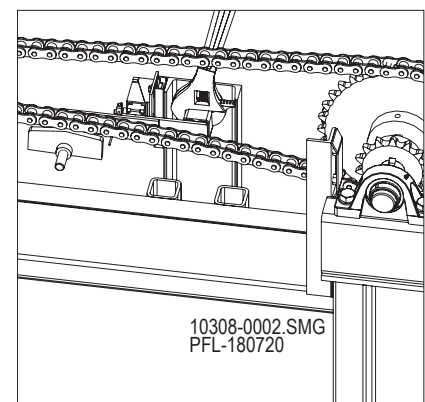
Adjust Drive Chain Tensioner Figure 12-54
