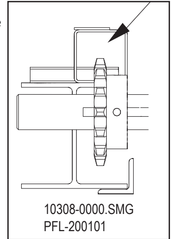
Center the Lift Chain Down the Chain Tube and Tighten Setscrews Figure 12-42
