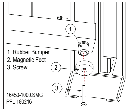
Attach Panel Magnetic Foot Figure 16-78
