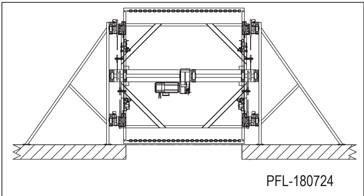
Facing a Mezzanine Figure 13-11
