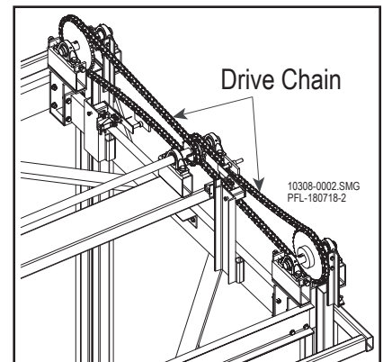
Install the Drive Chain Figure 12-38
