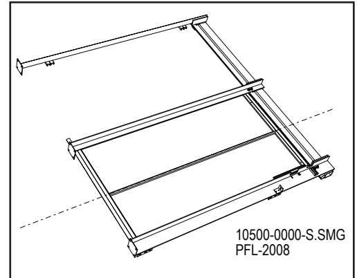
Mark Center Line of Sliding Gate Layout Figure 16-3
