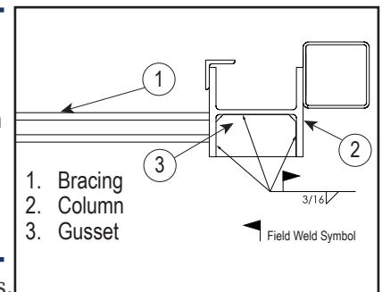
Bracing Columns Figure 13-4
