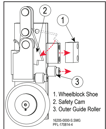
Rotate the Safety Cam Figure 12-11
