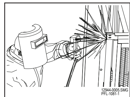
Weld Gate Header to Gate Posts Figure 16-27
