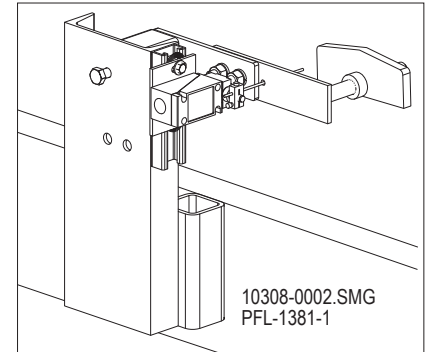
Assembled Drive Chain Tensioner Figure 12-53
