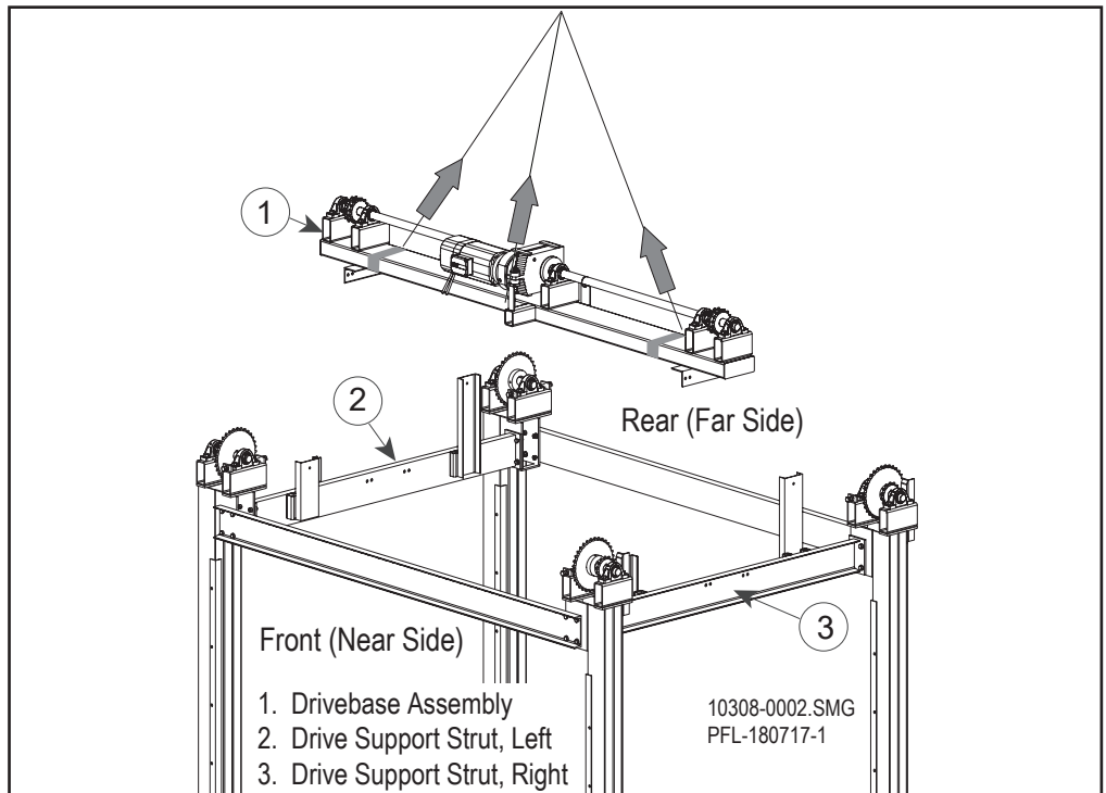
Drivebase Assembly Placement Figure 12-33
