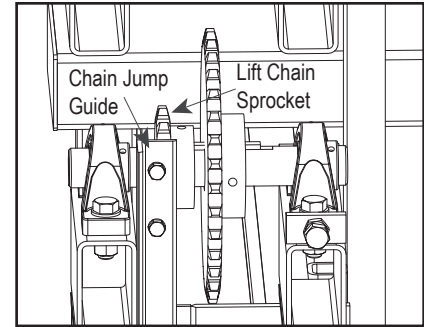
Reinstall the Chain Jump Guides Figure 12-55
