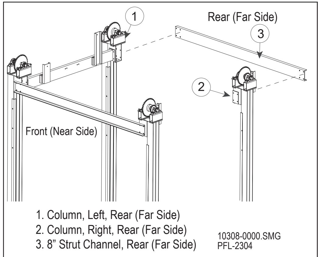
Attach Strut Channel Figure 12-27
