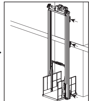
Attach Limit Switches
