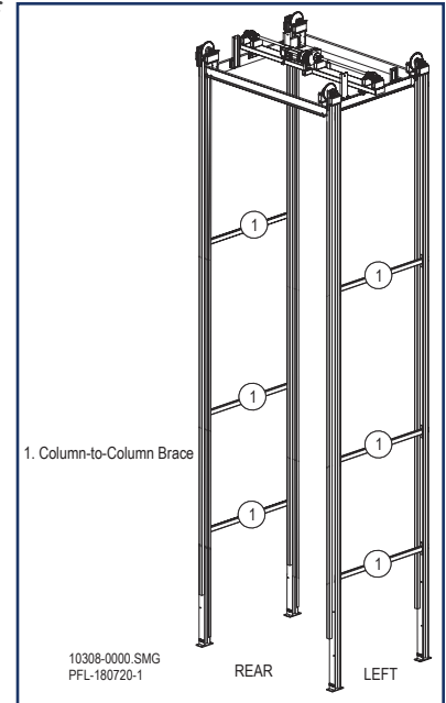
Bracing Example Figure 12-34
