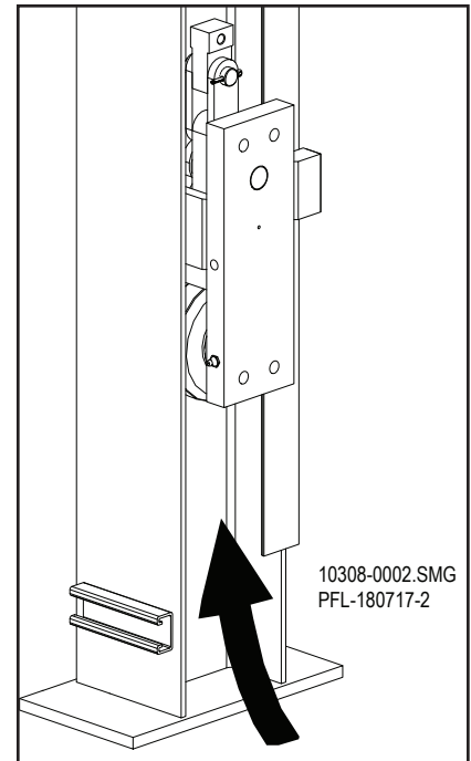
Insert Wheelblock Figure 12-14
