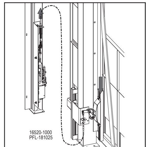
Pelle Interlock Figure 17-7
