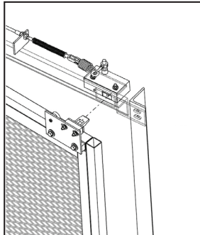
Install Interlocks
