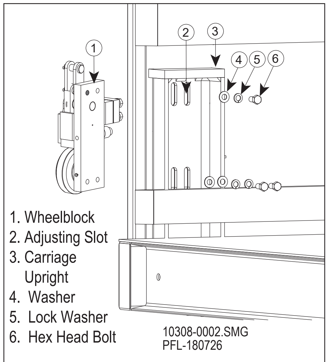
Wheelblock Mounting Figure 12-16
