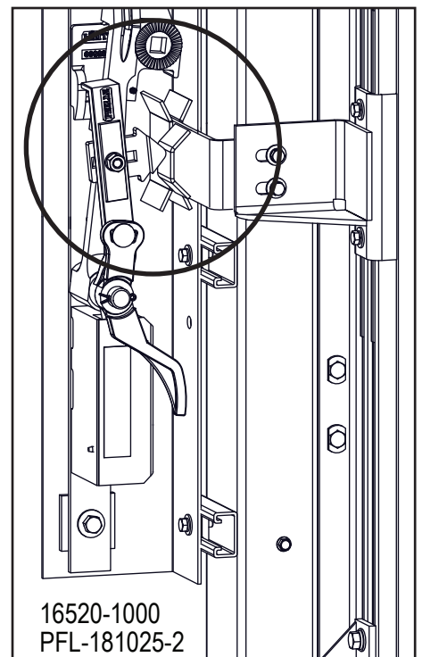
Peelle Interlock Closed Position Figure 17-9
