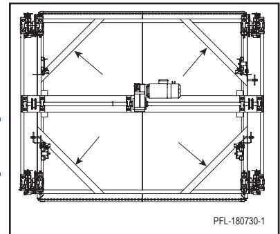
Weld Corner Braces Figure 12-35
