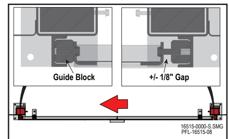
Guide Block Gap 16-61
