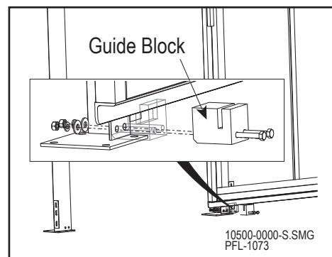
Bolt Guide Block Figure 16-2
