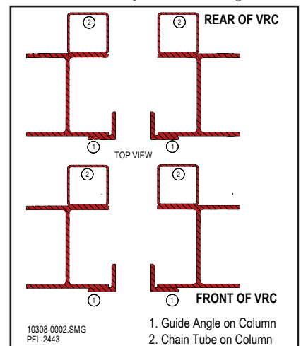
Verify Orientation Figure 12-3
