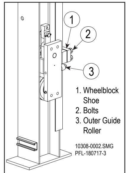
Reattach Shoe and Roller Figure 12-15
