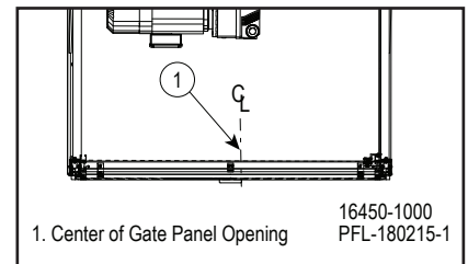
Alignment Figure 16-63
