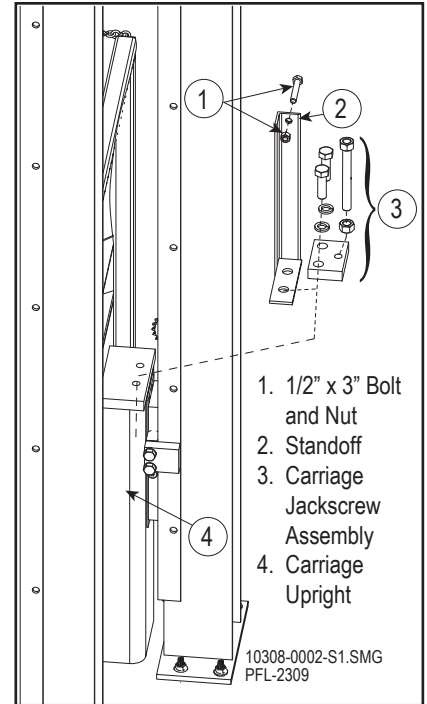
Assemble the Standoff and Jackscrew Figure 12-44
