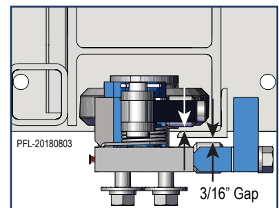
Verify Gap Figure 12-20
