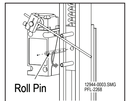
Limit Switch Adjustment Figure 12-50
