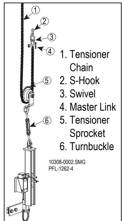
Chain Tensioner Assembly Figure 12-47
