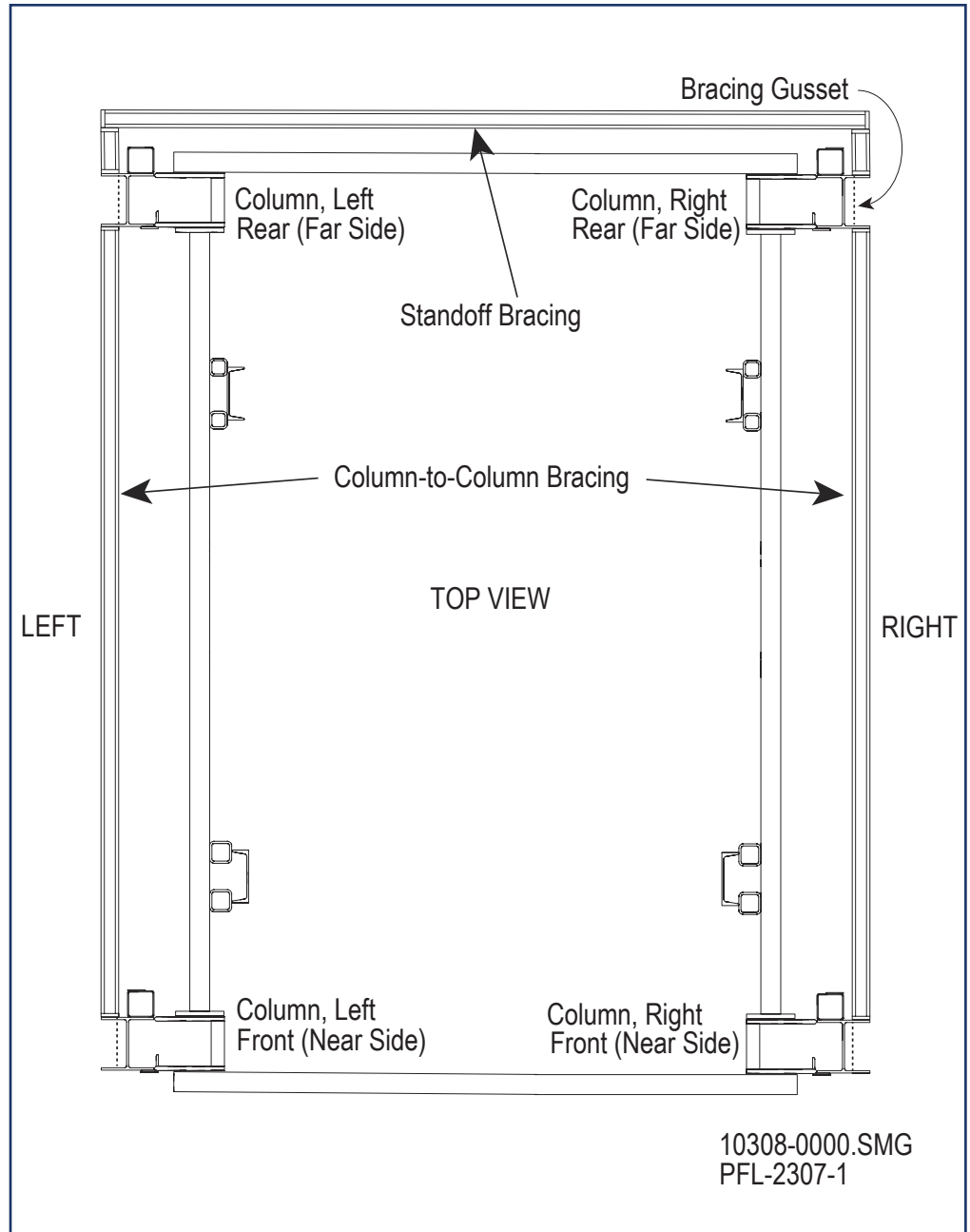
Standoff Bracing Figure 13-16
