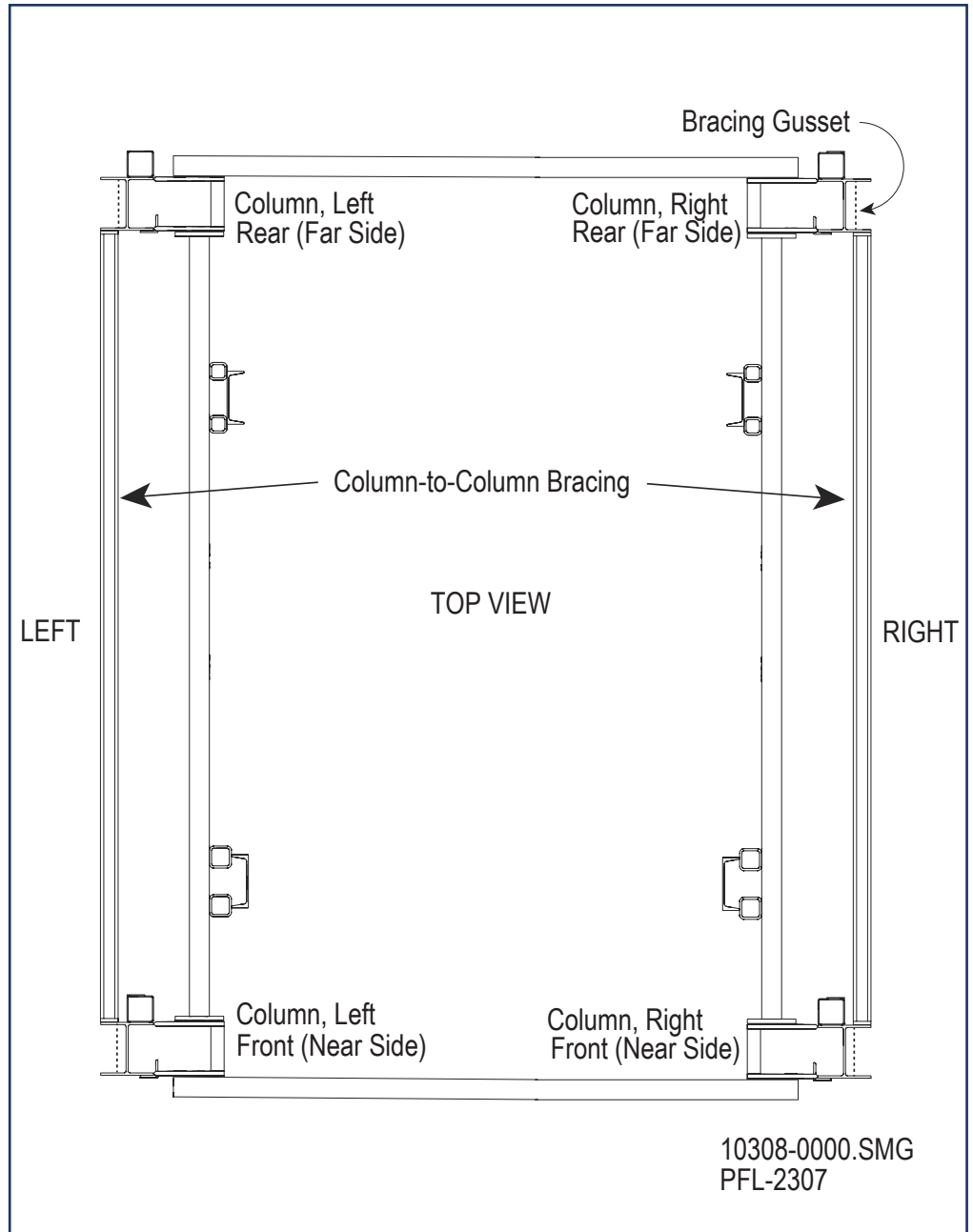
Column-to-Column Bracing Figure 13-15
