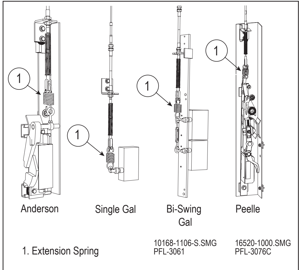
Cable Interlocks Figure 17-1
