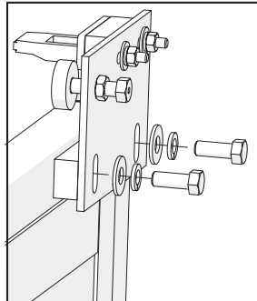
Install Keepers
