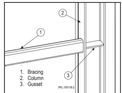
Bracing Columns Figure 13-3
