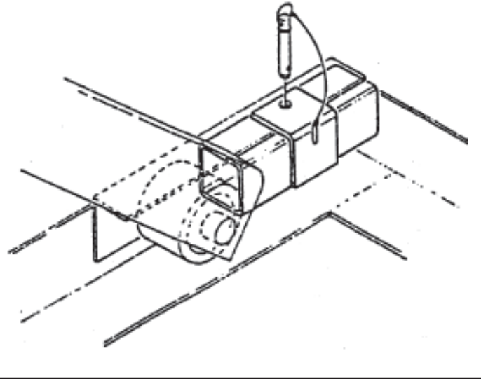
FIGURE 1: MAINTENANCE CHOCK
