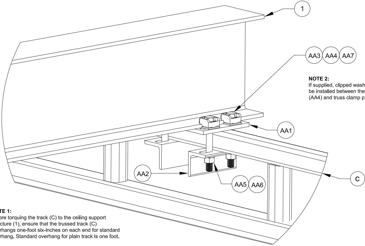
Detail "AA" (Track to Ceiling Support Structure Using Flush-Cross Mount Hanger)
