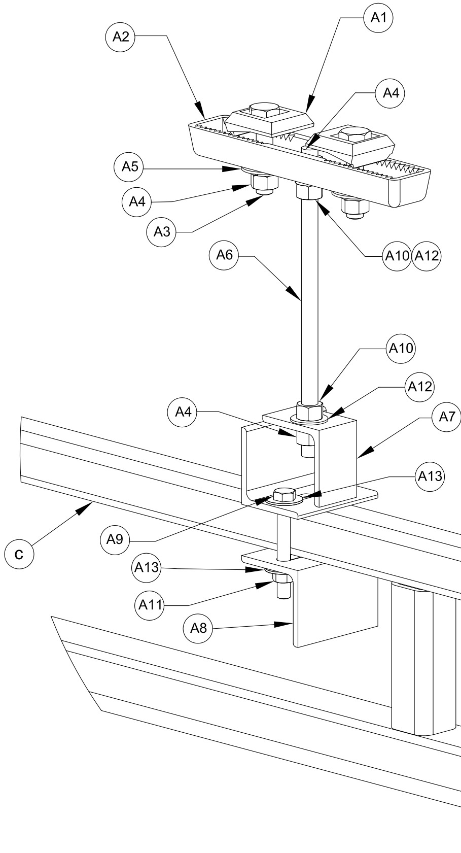
Detail "A" (Track to Ceiling Support Structure Using Drop Rod Hanger)
