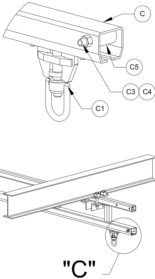
Detail "C" (Trolley[s] and End Stops to Track)
