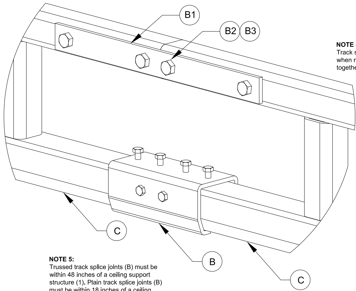
Detail "B" (Track Splice to Track Sections)
