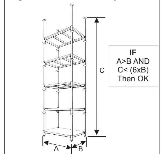
Figure 5: Maximum stack height
