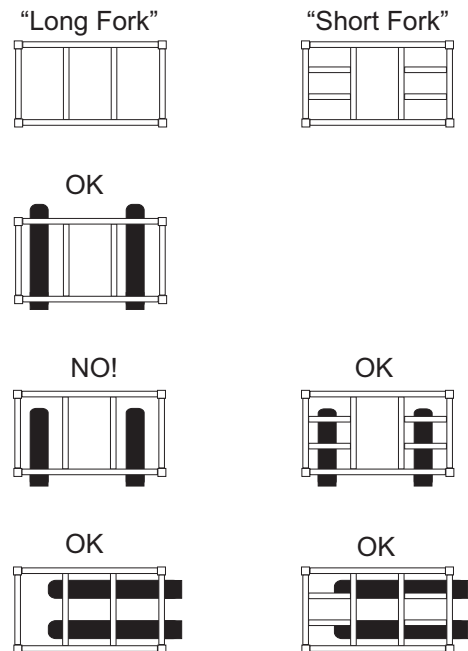
Figure 3: Stac-King base Vs Fork length
