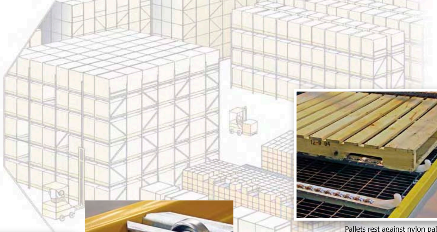
Pallets rest against nylon pallet stop Optional steel pallet stops available
