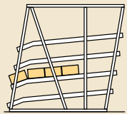
10° layback vertical frame with carton tilt shelves.
