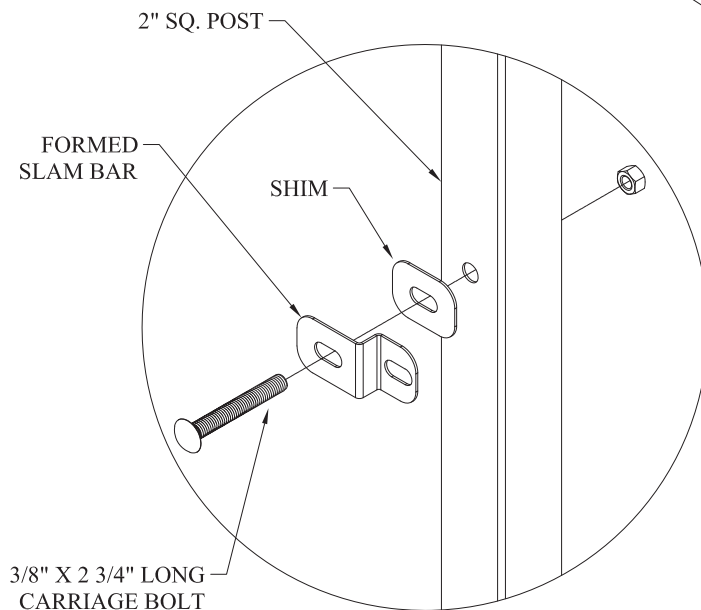
SLAM BARS
