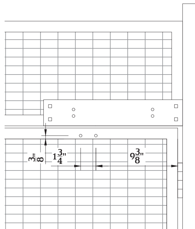
Fig.2 Inside Swing
