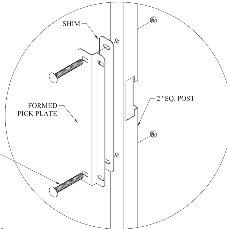
PICK PLATE
