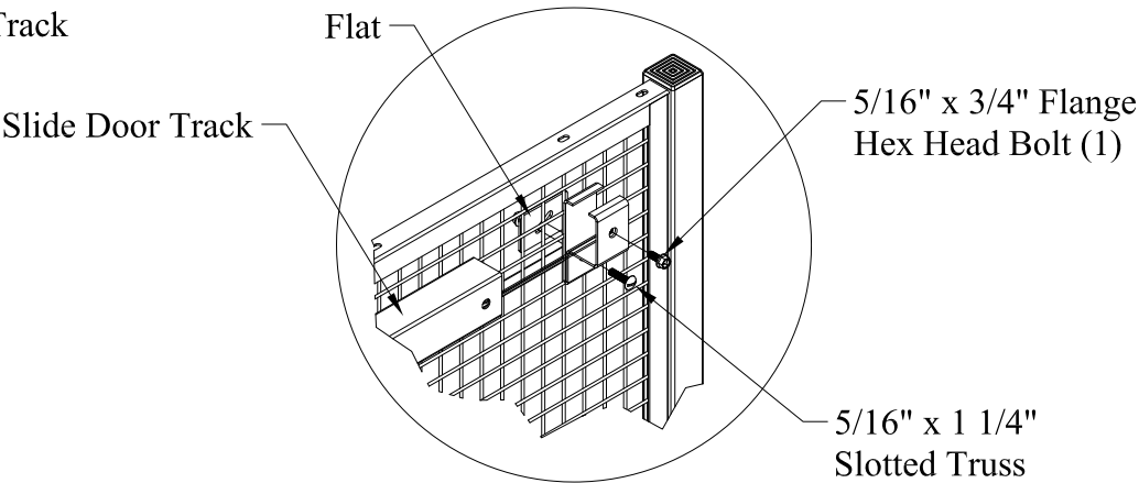
Single Track Bracket to Mesh
