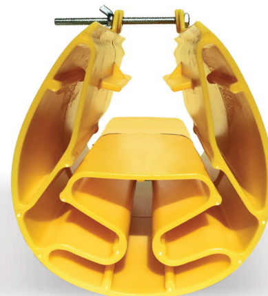
YJ-3x1-5/8 Fits 3"x 1-5/8" Rack
